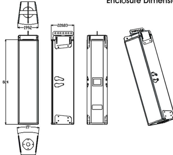
Enclosure Dimension :
